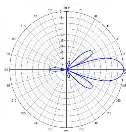
Horizontal Polarisation / Horizontal Plane
