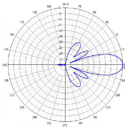
Vertical Polarisation / Horizontal Plane
